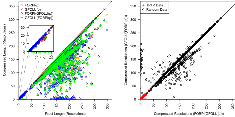
(a) Compressed length vs. input length. (b) FORPI(GFOLU(p)) vs. GFOLU(FORPI(p)).
