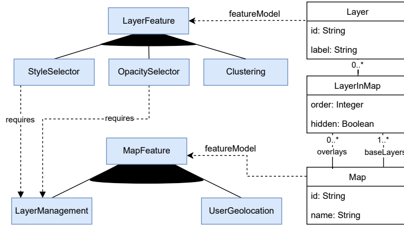
Figure 2: Example of the feature's integration in the DSL model
