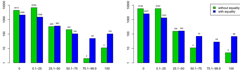
Figure 1: Histogram of problems by the percentage of blocked clauses eliminated. BCE applied after simple clasification (left) and after clasification preceded by PPE and UDE (right).
