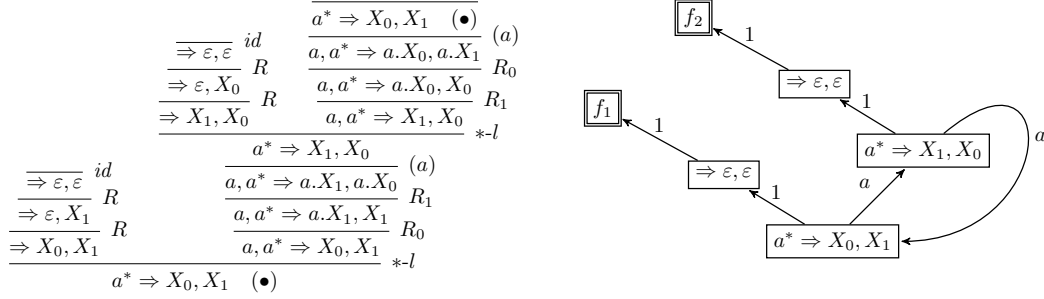
Figure 3: The synchronised proof \Pi_0 \times \Pi_1 and its automaton (Ex. 7, 18, 21).
