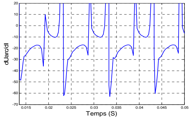
Fig. II (f): the resistance of arc For a frequency 50Hz
