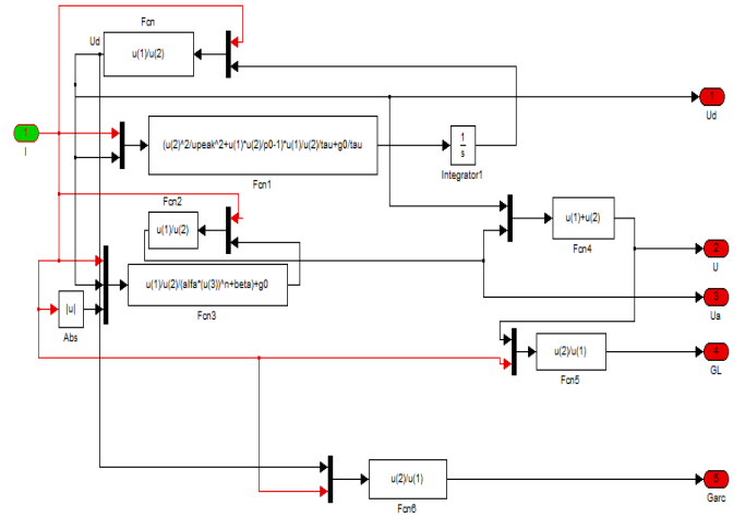
Fig. 1. Universal simulation scheme of a discharge lamp[6], [7], [8].
