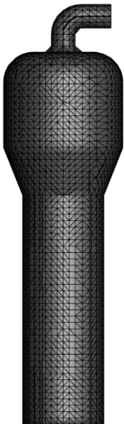
Figure 7. The meshed geometry with the expanded cross-sectional area on top
