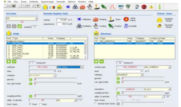
Fig. 2: TRNBUILD mechanism
