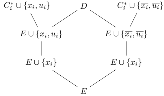
■ Figure 7 Q-Res derivation of the resolvent E from \text{EQ} \times_i^* .
