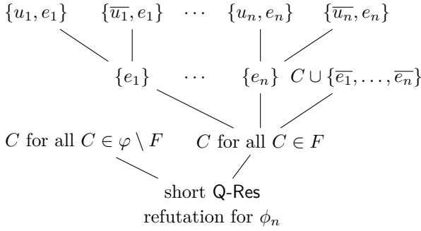
■ Figure 8 Polynomial-size QU-Res refutations for \phi^* .
