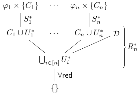
■ Figure 3 Polynomial-size LD-Q-Res refutations for \chi_n^\Phi .
