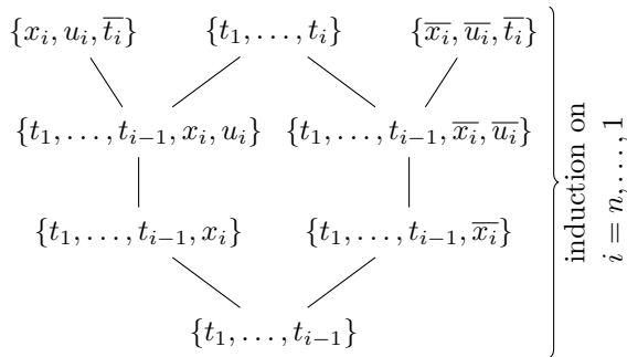
■ Figure 4 Polynomial-size Q-Res refutation of {}^{11}\text{SC}_n^{\text{EQ}} .
