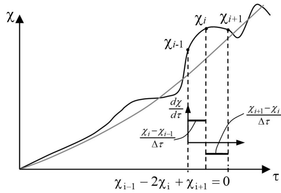
Fig. 4. Idea of linear regularization of solution \chi(\tau)
