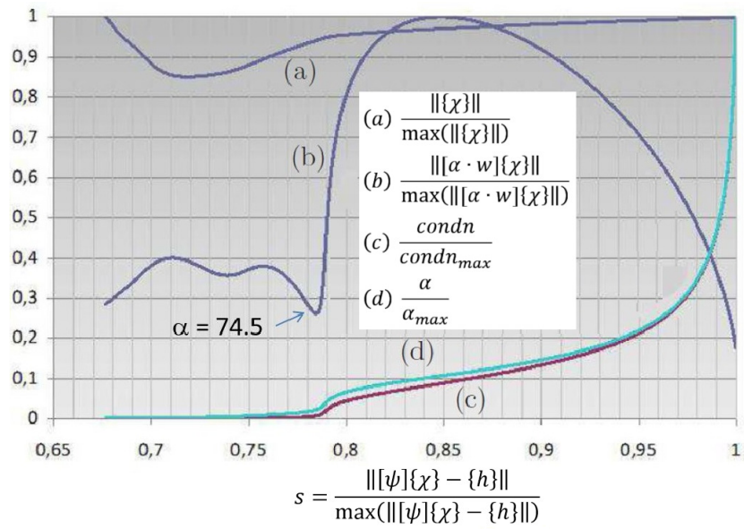
Fig. 8. Dimensionless distributions of: \|[\alpha \cdot w]\{\chi\}\| / \max(\|[\alpha \cdot w]\{\chi\}\|) , \alpha/\alpha_{max} , \|\chi\| / \max \|\chi\| , condn/condn_{max} , as function of dimensionless values
