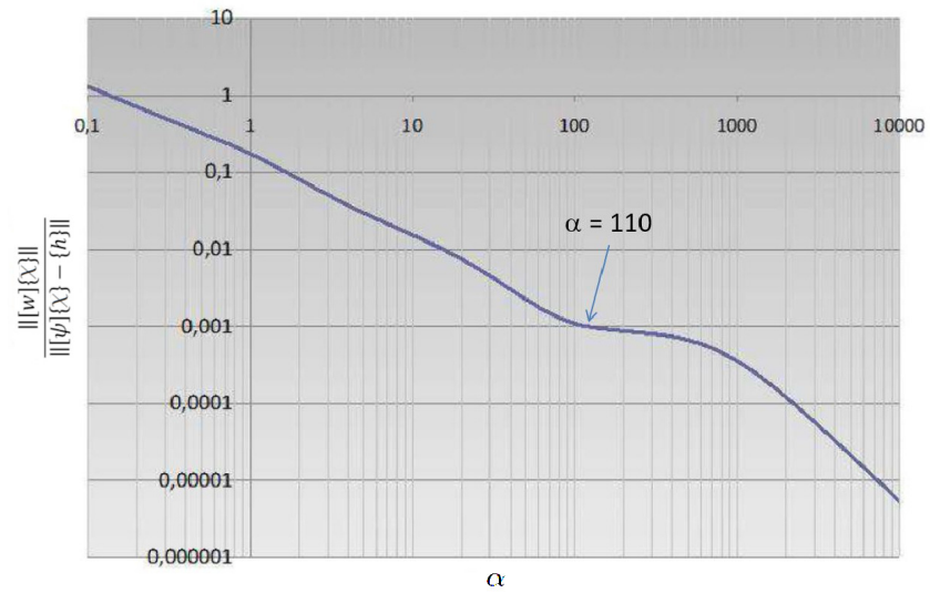
Fig. 7. L - curve in coordinates (\alpha, \frac{\|w\{x}\|}{\|\psi\{x\} - \{h\}\|})
