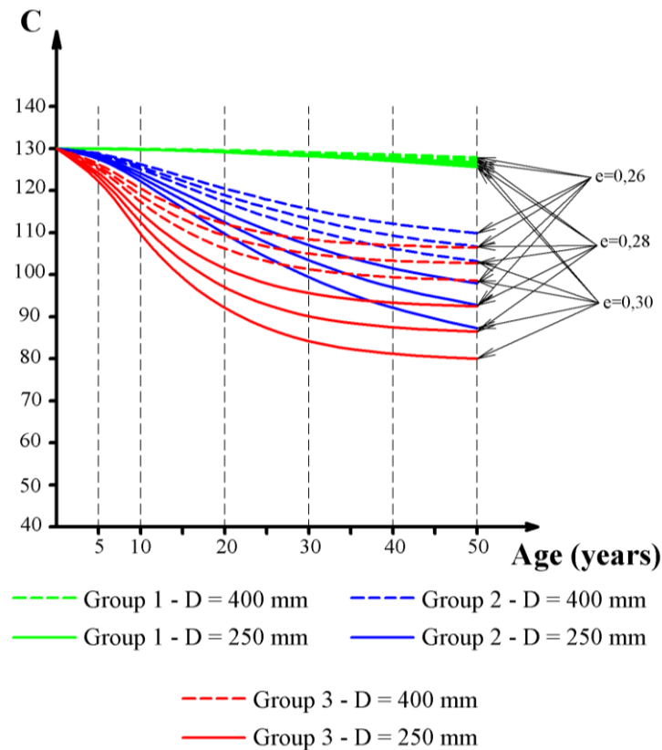
Figure 3. Change in the roughness coefficient C of pipes with internal cement coatings from the age of their operation and the characteristics of natural waters.
