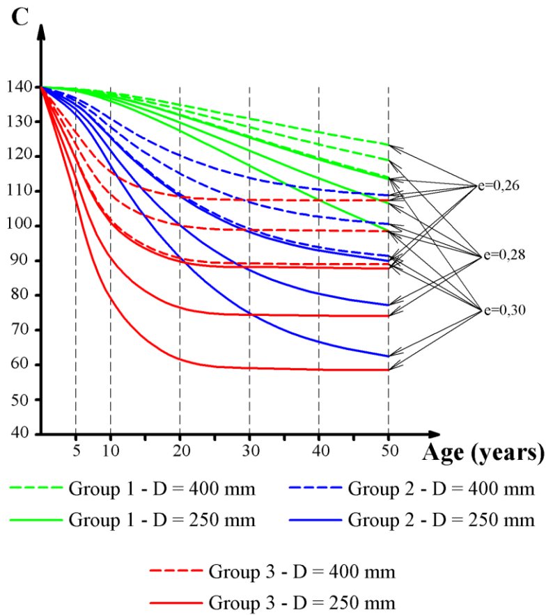
Figure 2. Change in the roughness coefficient C of steel pipes from the age of their operation and the characteristics of natural waters.
