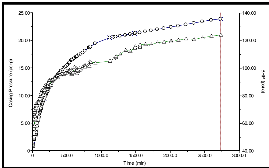
Fig. 7. Casing Pressure (circles) and BHP (triangles) vs Time Source: TWM Software., 2019
