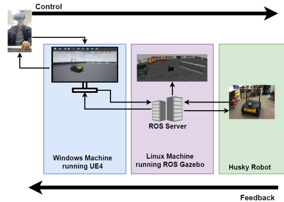
Figure 2: Block Diagram of Teleoperation System
